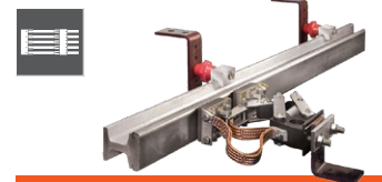
Non-insulated conductor rails
